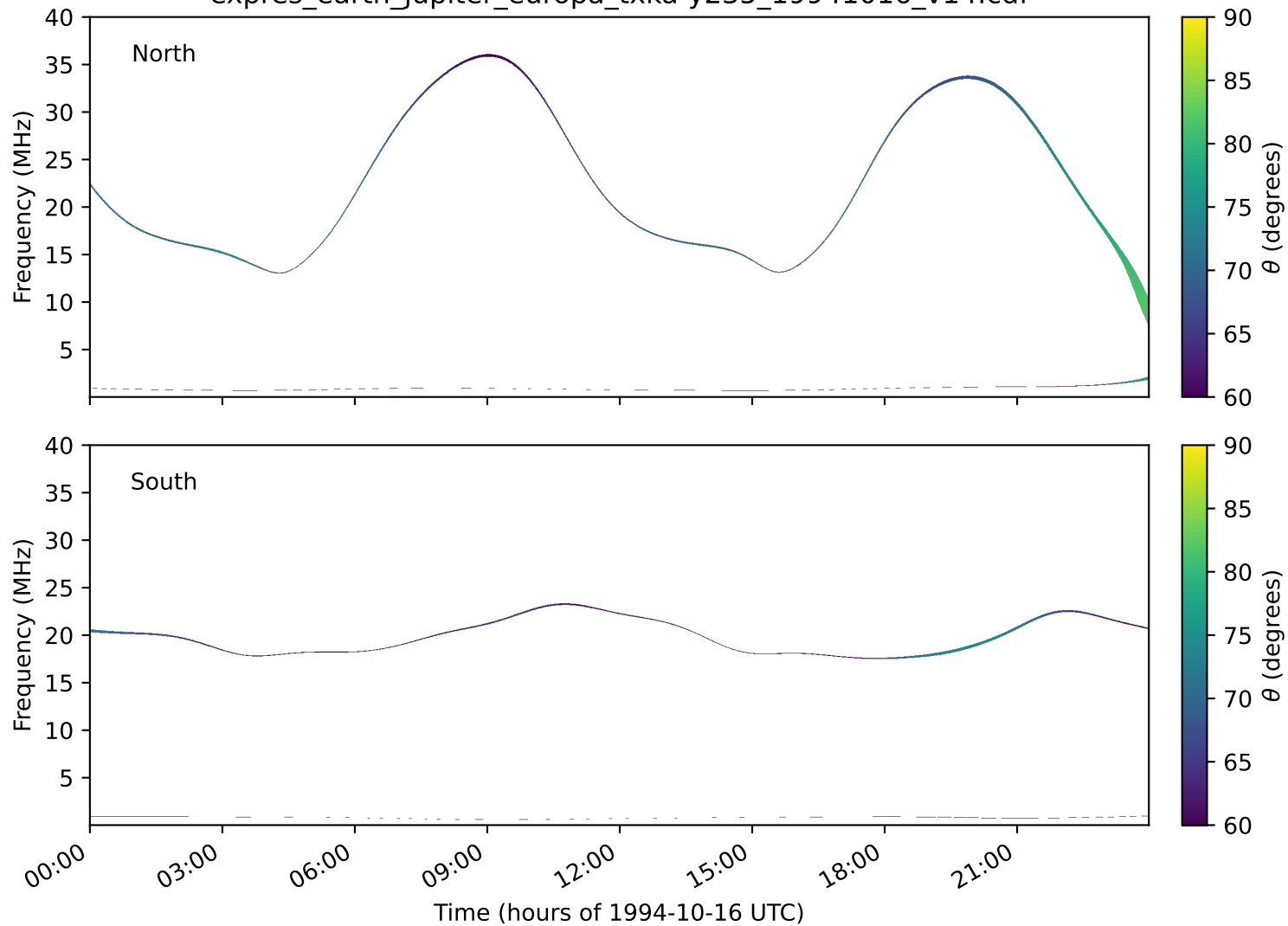
expres_earth_jupiter_europa_txka-y235_19941016_v14.cdf
