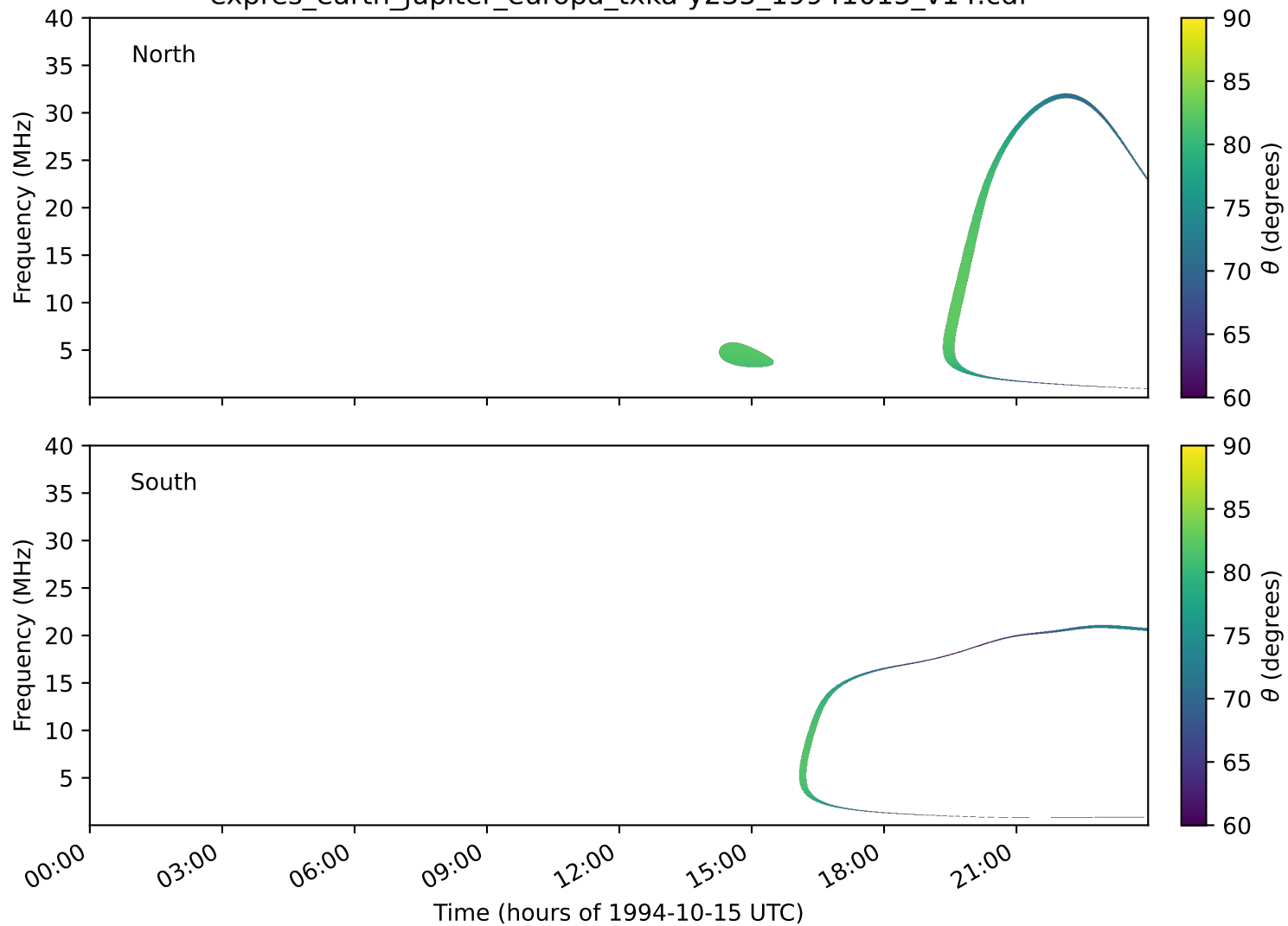
expres_earth_jupiter_europa_txka-y235_19941015_v14.cdf
