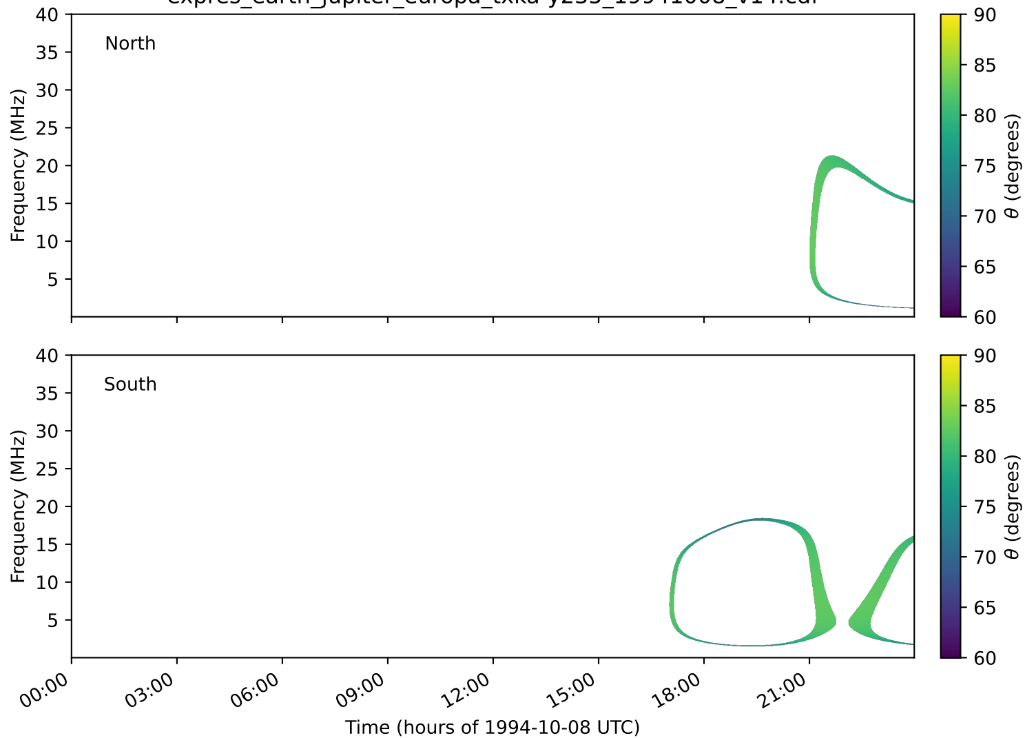
expres_earth_jupiter_europa_txka-y235_19941008_v14.cdf
