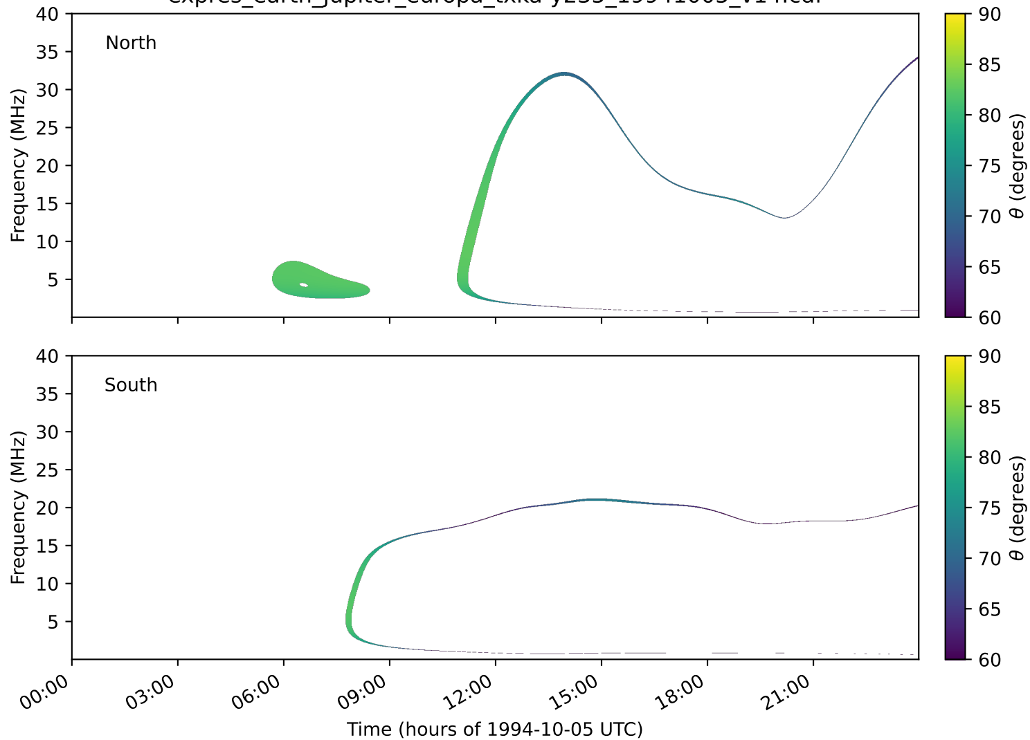
expres_earth_jupiter_europa_txka-y235_19941005_v14.cdf
