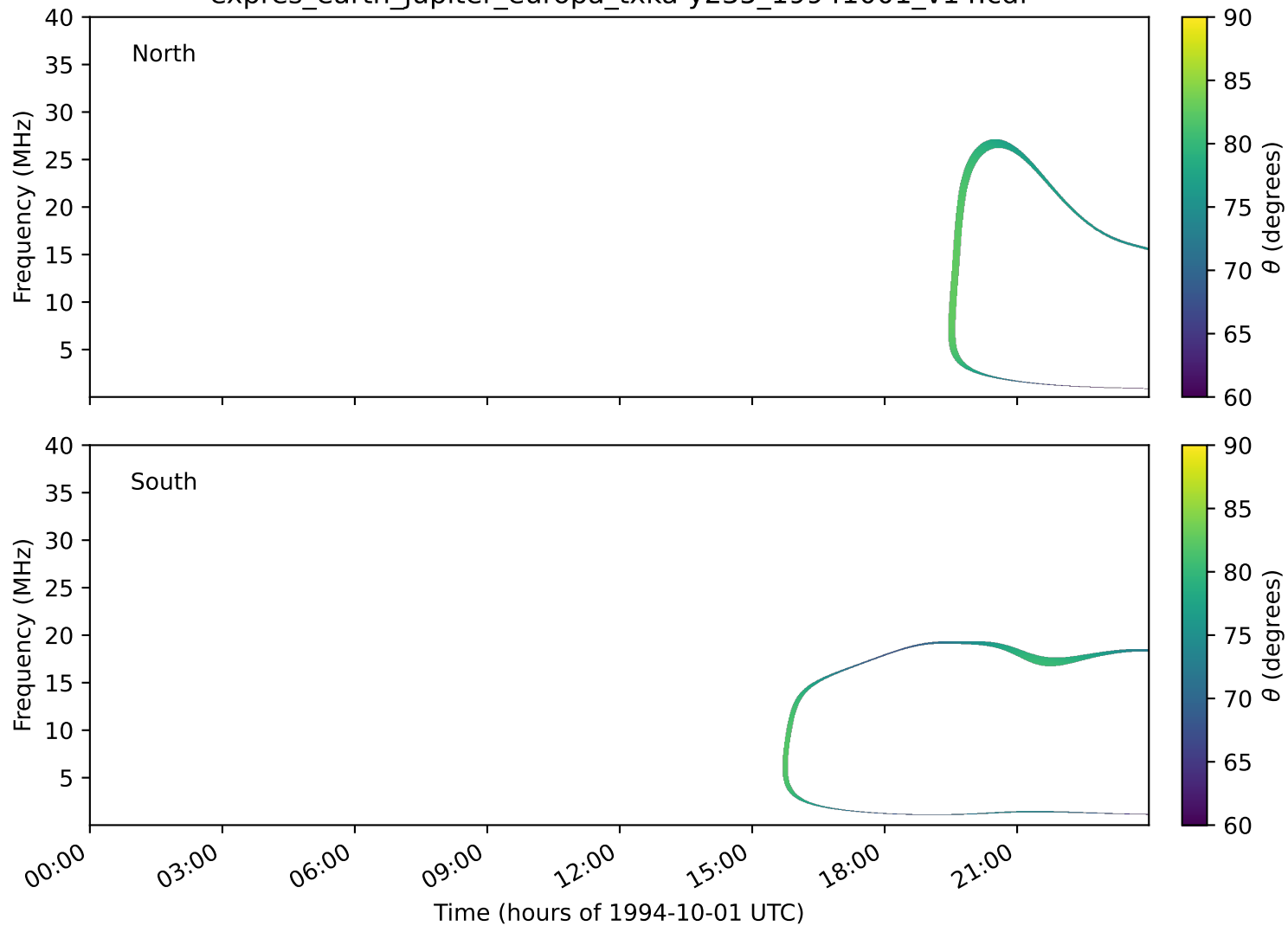
expres_earth_jupiter_europa_txka-y235_19941001_v14.cdf
