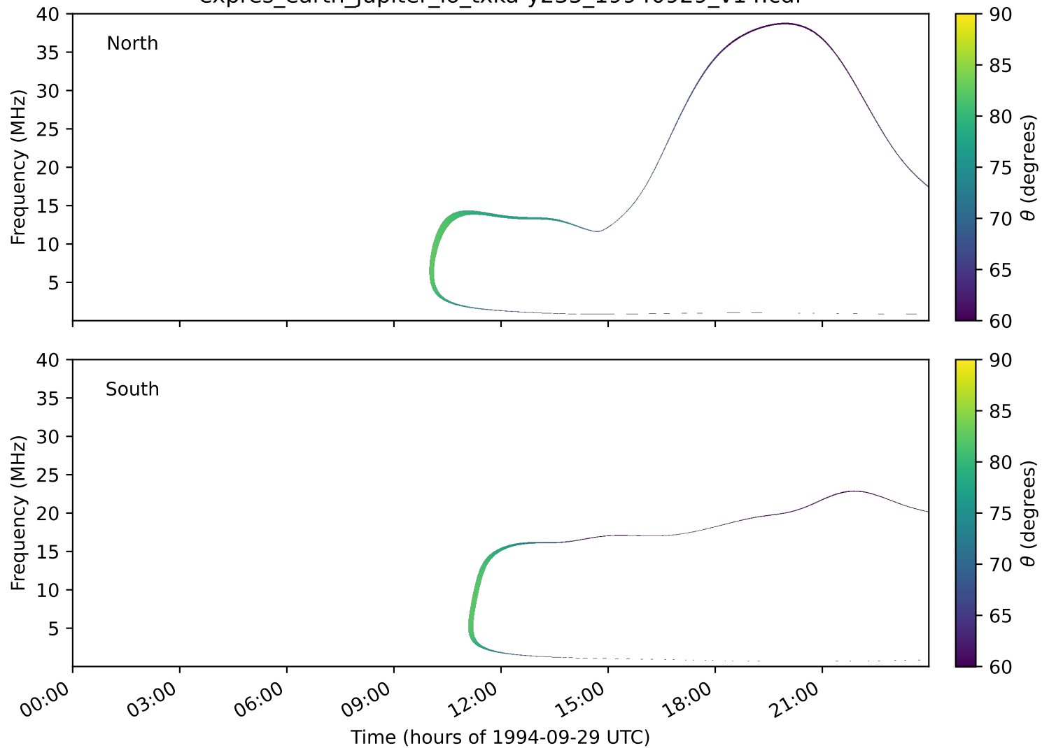
expres_earth_jupiter_io_txka-y235_19940929_v14.cdf
