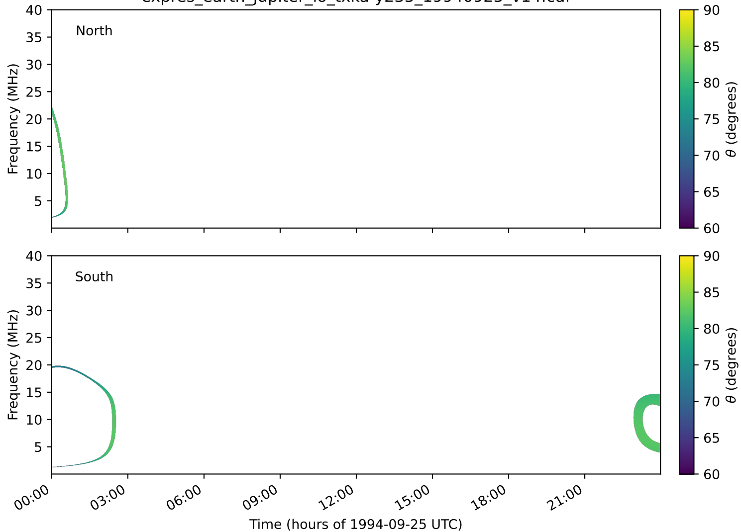
expres_earth_jupiter_io_txka-y235_19940925_v14.cdf
