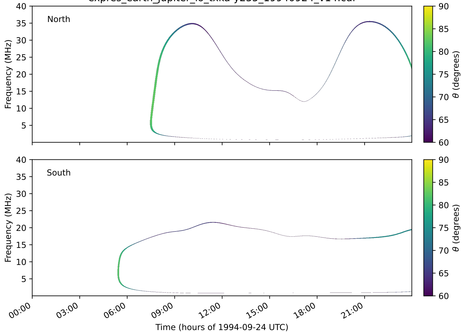
expres_earth_jupiter_io_txka-y235_19940924_v14.cdf
