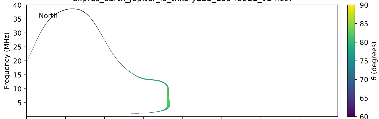
expres_earth_jupiter_io_txka-y235_19940921_v14.cdf
