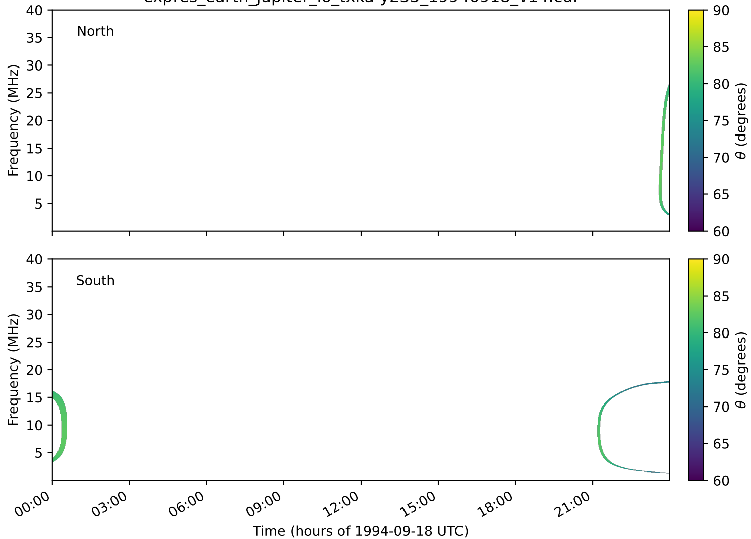
expres_earth_jupiter_io_txka-y235_19940918_v14.cdf
