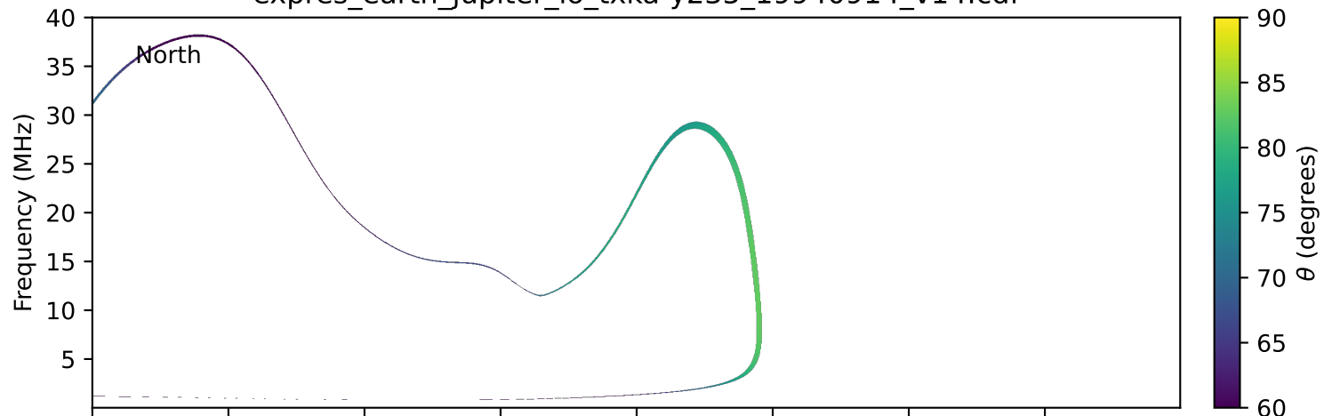
expres_earth_jupiter_io_txka-y235_19940914_v14.cdf
