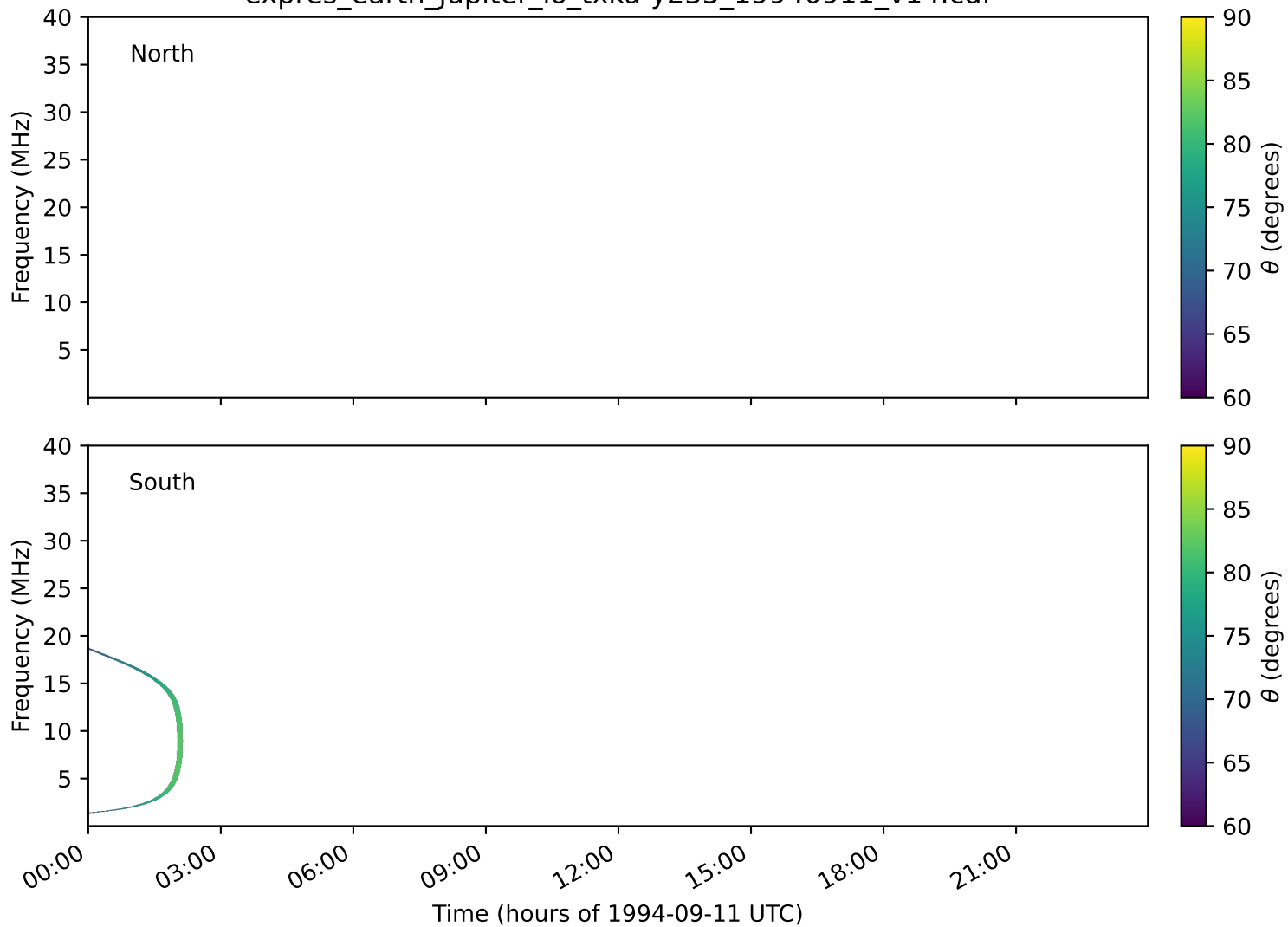
expres_earth_jupiter_io_txka-y235_19940911_v14.cdf
