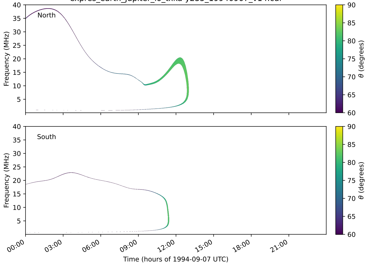
expres_earth_jupiter_io_txka-y235_19940907_v14.cdf
