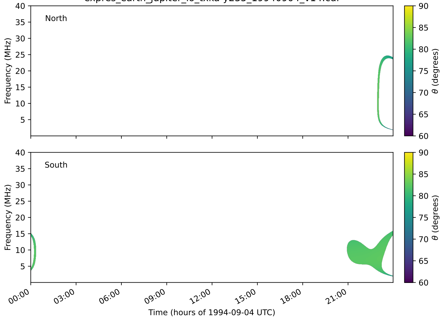
expres_earth_jupiter_io_txka-y235_19940904_v14.cdf
