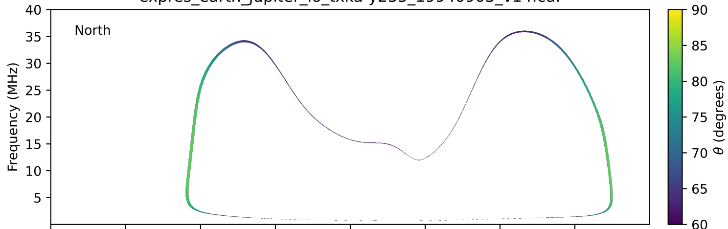
expres_earth_jupiter_io_txka-y235_19940903_v14.cdf
