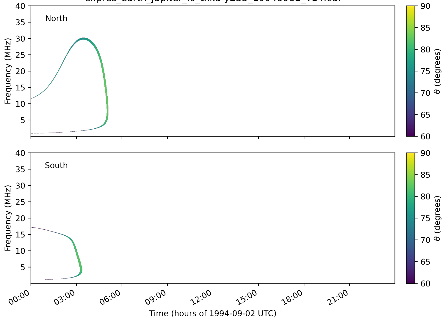
expres_earth_jupiter_io_txka-y235_19940902_v14.cdf
