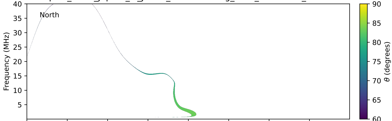
expres_earth_jupiter_io_jrm33_lossc-wid1deg_3kev_19940921_v11.cdf
