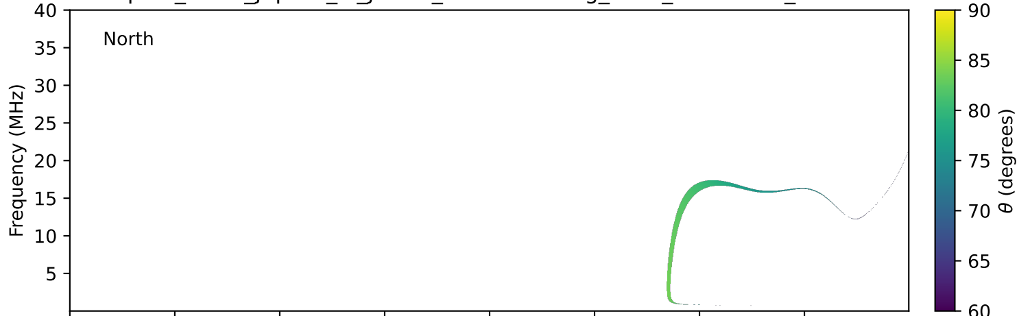
expres_earth_jupiter_io_jrm33_lossc-wid1deg_3kev_19940920_v11.cdf
