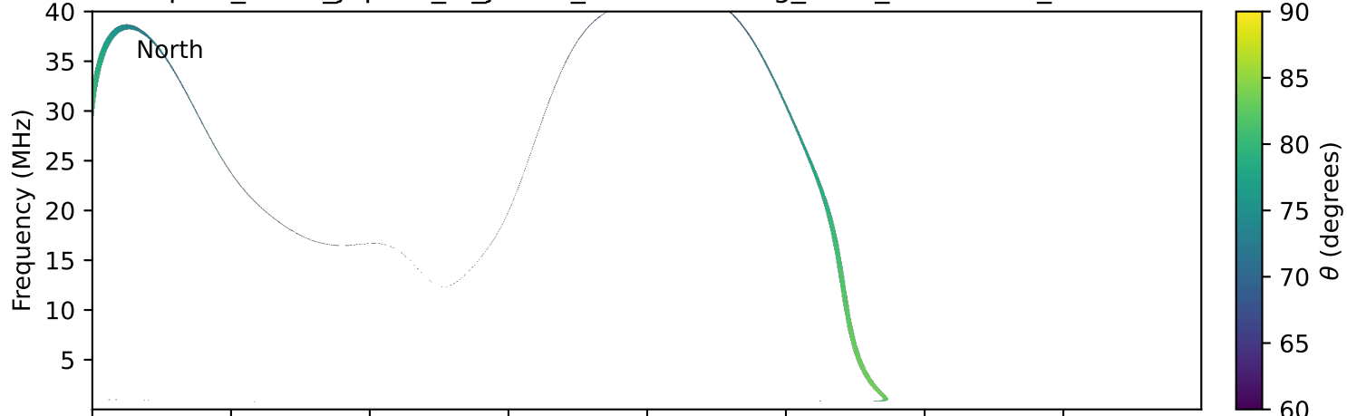
expres_earth_jupiter_io_jrm33_lossc-wid1deg_3kev_19940919_v11.cdf
