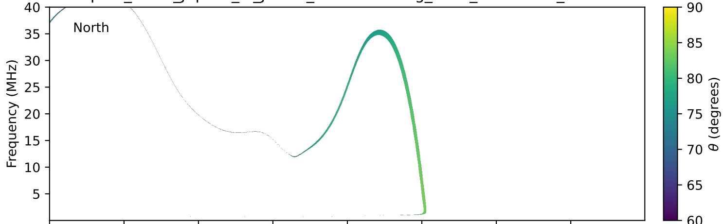
expres_earth_jupiter_io_jrm33_lossc-wid1deg_3kev_19940914_v11.cdf
