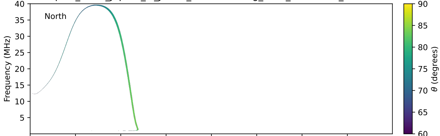
expres_earth_jupiter_io_jrm33_lossc-wid1deg_3kev_19940909_v11.cdf
