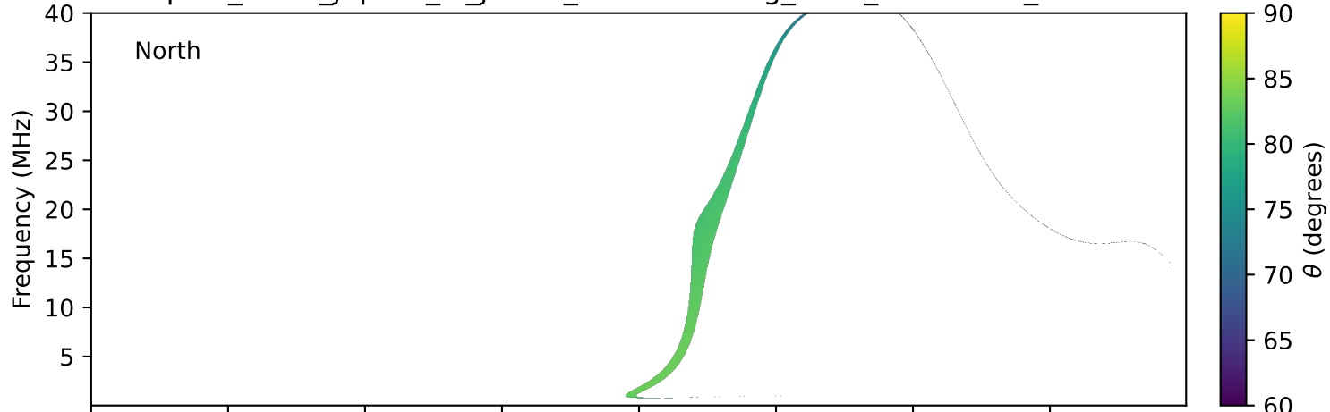
expres_earth_jupiter_io_jrm33_lossc-wid1deg_3kev_19940908_v11.cdf
