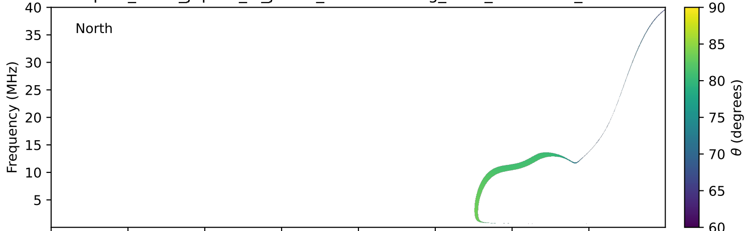
expres_earth_jupiter_io_jrm33_lossc-wid1deg_3kev_19940906_v11.cdf
