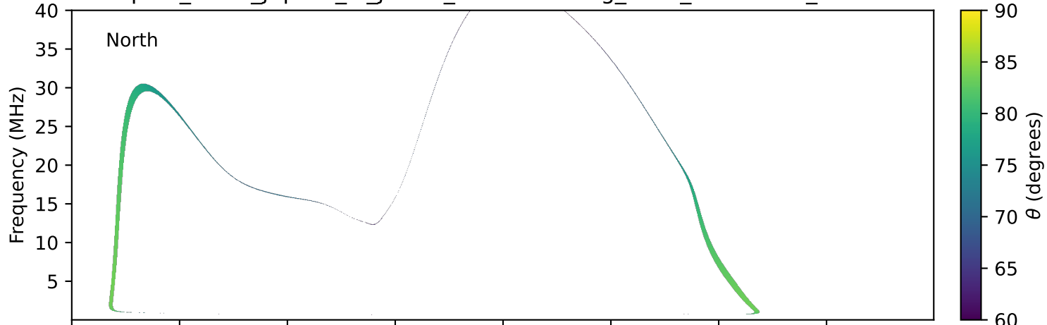
expres_earth_jupiter_io_jrm09_lossc-wid1deg_3kev_19940926_v11.cdf
