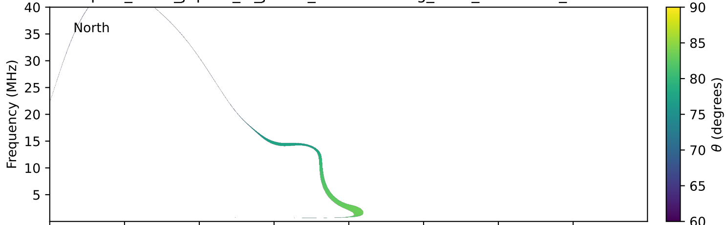
expres_earth_jupiter_io_jrm09_lossc-wid1deg_3kev_19940921_v11.cdf
