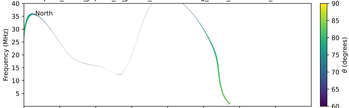
expres_earth_jupiter_io_jrm09_lossc-wid1deg_3kev_19940919_v11.cdf
