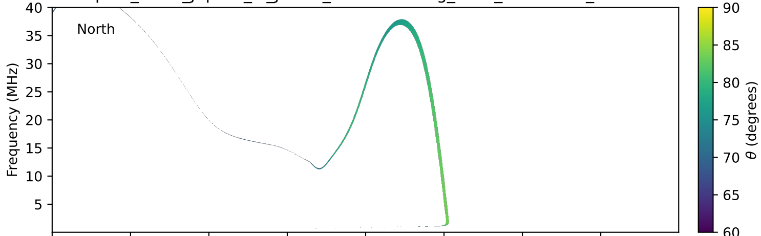
expres_earth_jupiter_io_jrm09_lossc-wid1deg_3kev_19940914_v11.cdf
