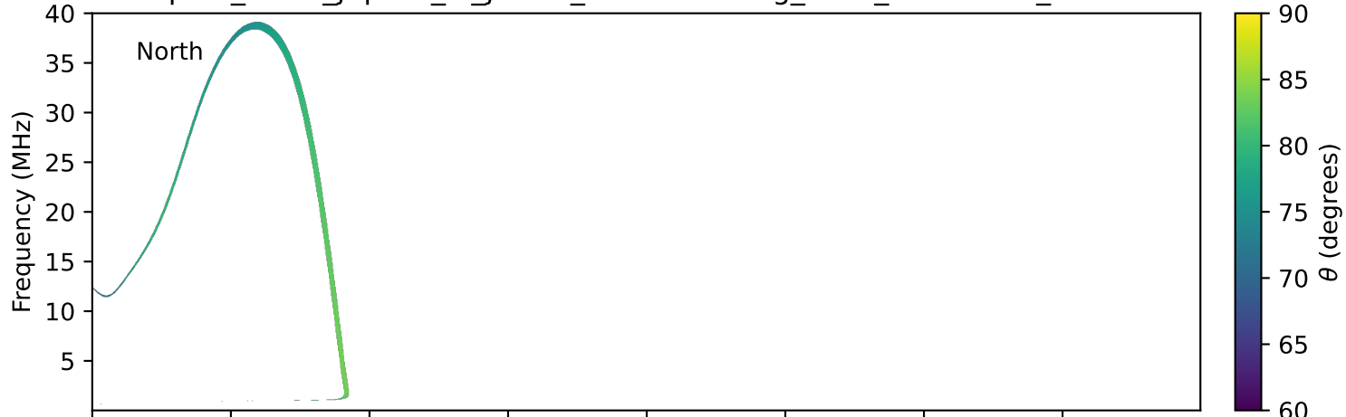
expres_earth_jupiter_io_jrm09_lossc-wid1deg_3kev_19940902_v11.cdf
