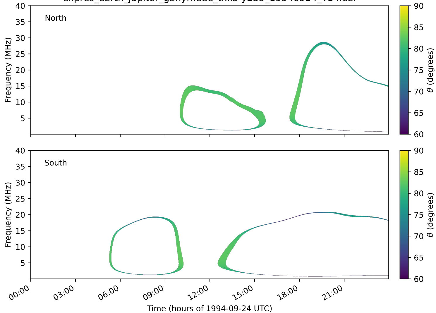
expres_earth_jupiter_ganymede_txka-y235_19940924_v14.cdf
