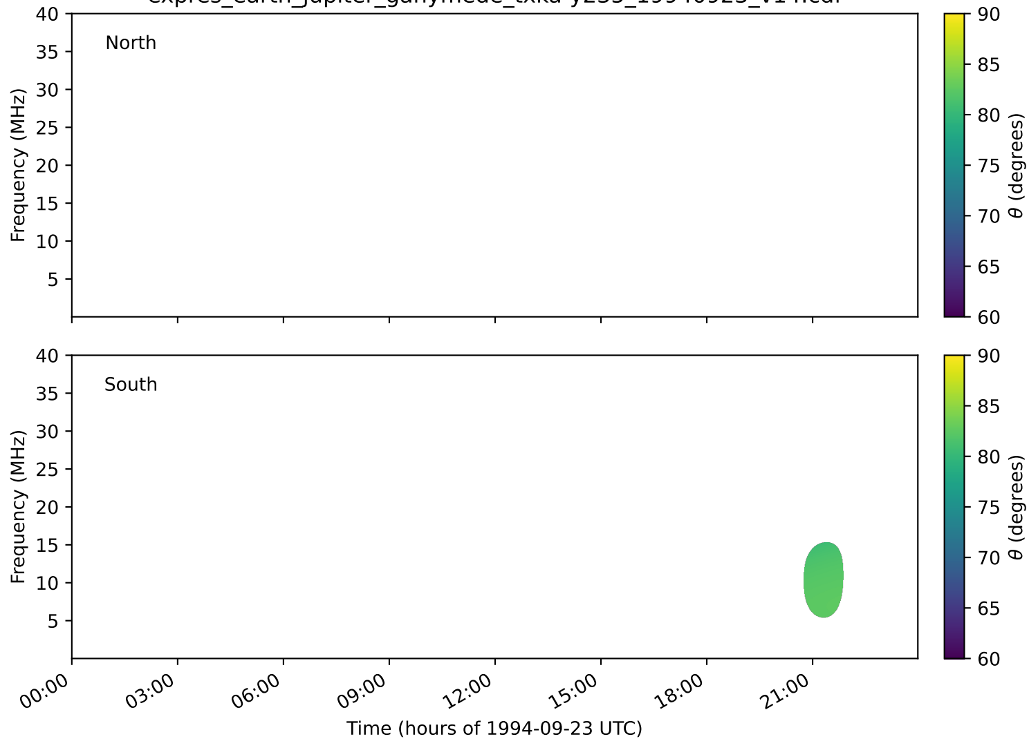
expres_earth_jupiter_ganymede_txka-y235_19940923_v14.cdf
