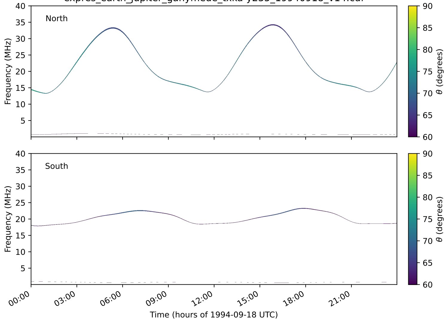
expres_earth_jupiter_ganymede_txka-y235_19940918_v14.cdf
