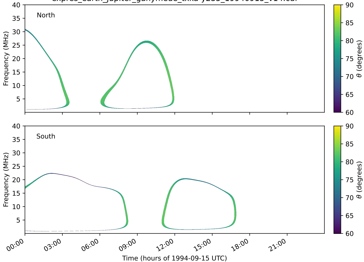
expres_earth_jupiter_ganymede_txka-y235_19940915_v14.cdf
