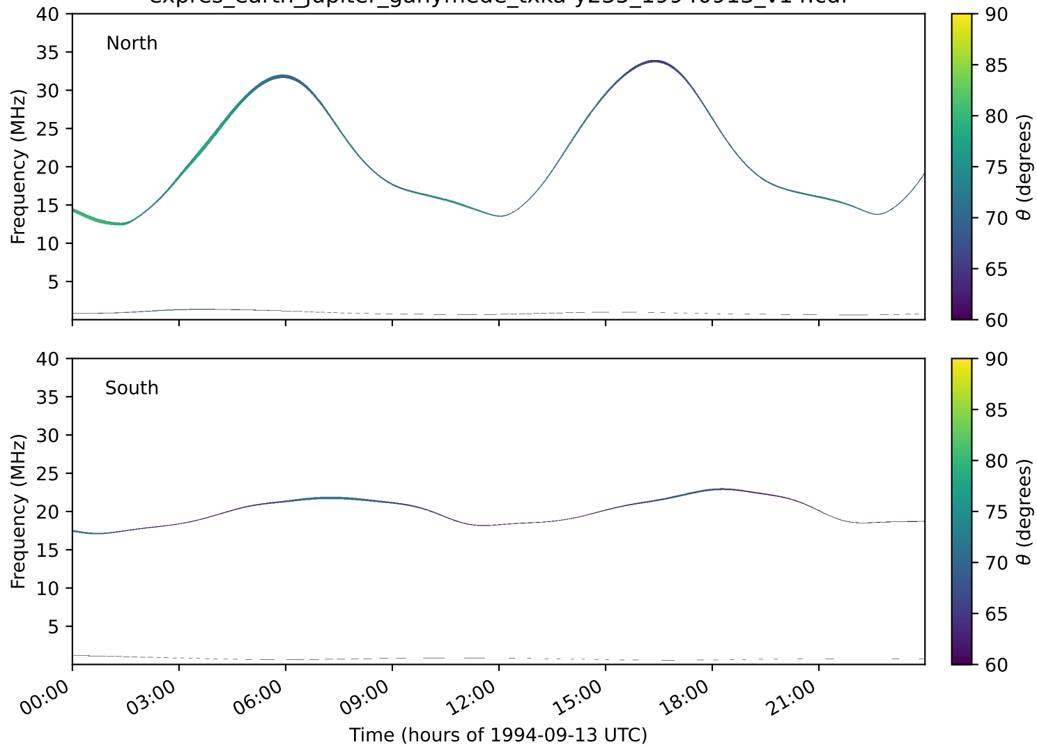
expres_earth_jupiter_ganymede_txka-y235_19940913_v14.cdf
