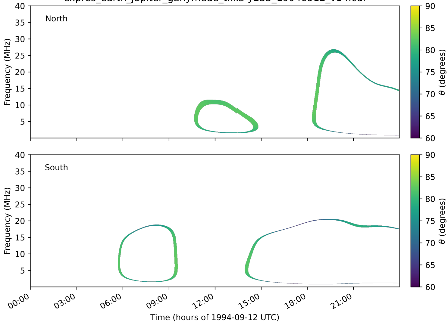
expres_earth_jupiter_ganymede_txka-y235_19940912_v14.cdf
