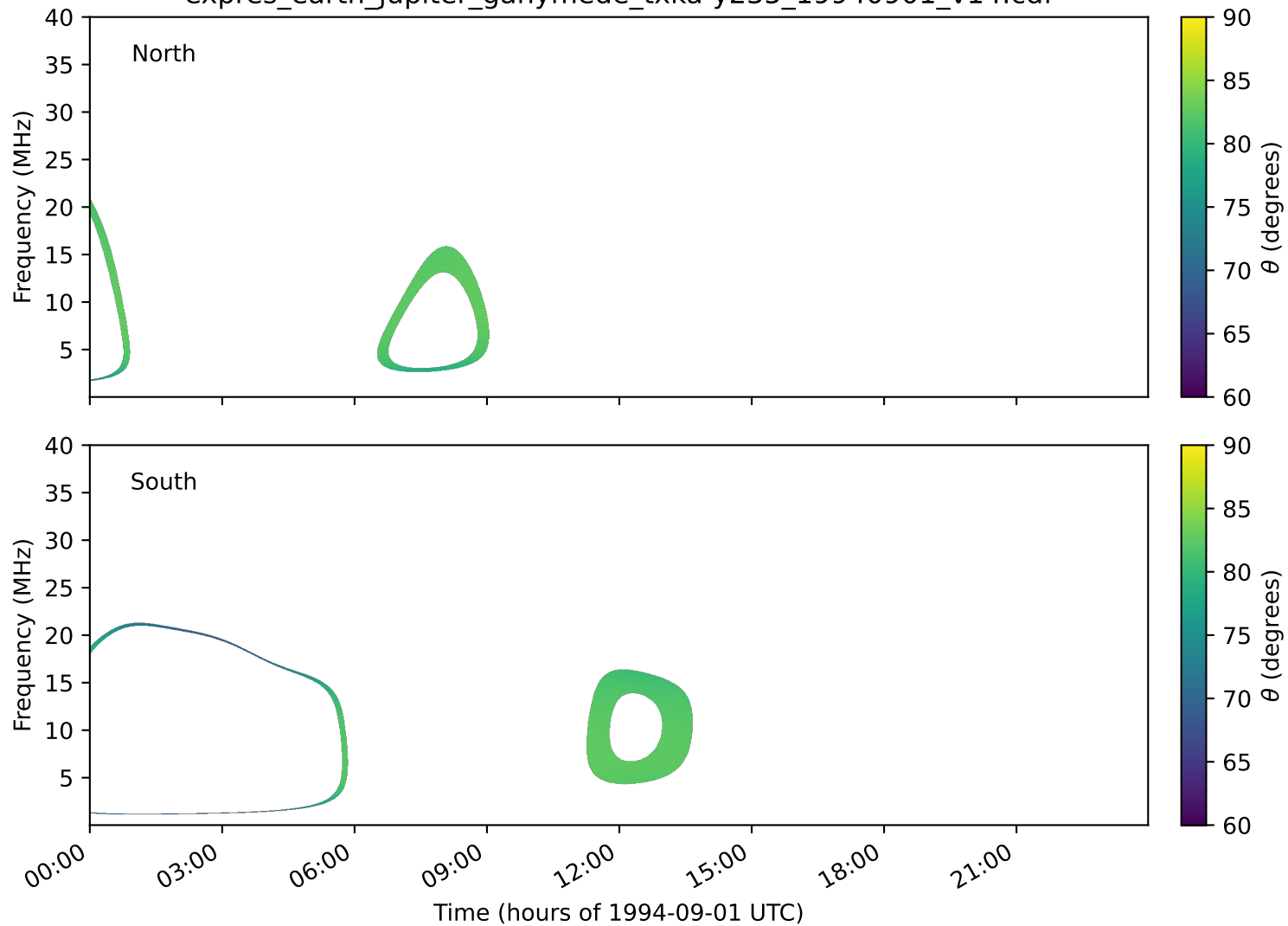
expres_earth_jupiter_ganymede_txka-y235_19940901_v14.cdf
