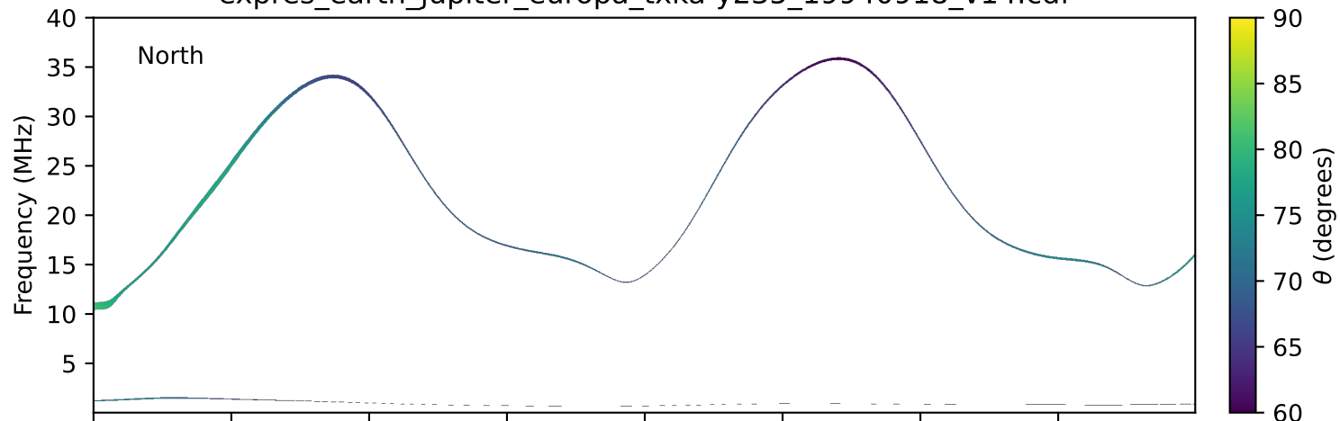
expres_earth_jupiter_europa_txka-y235_19940918_v14.cdf
