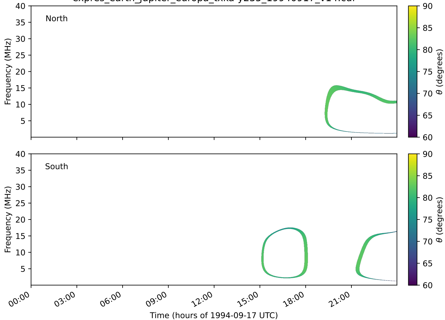
expres_earth_jupiter_europa_txka-y235_19940917_v14.cdf
