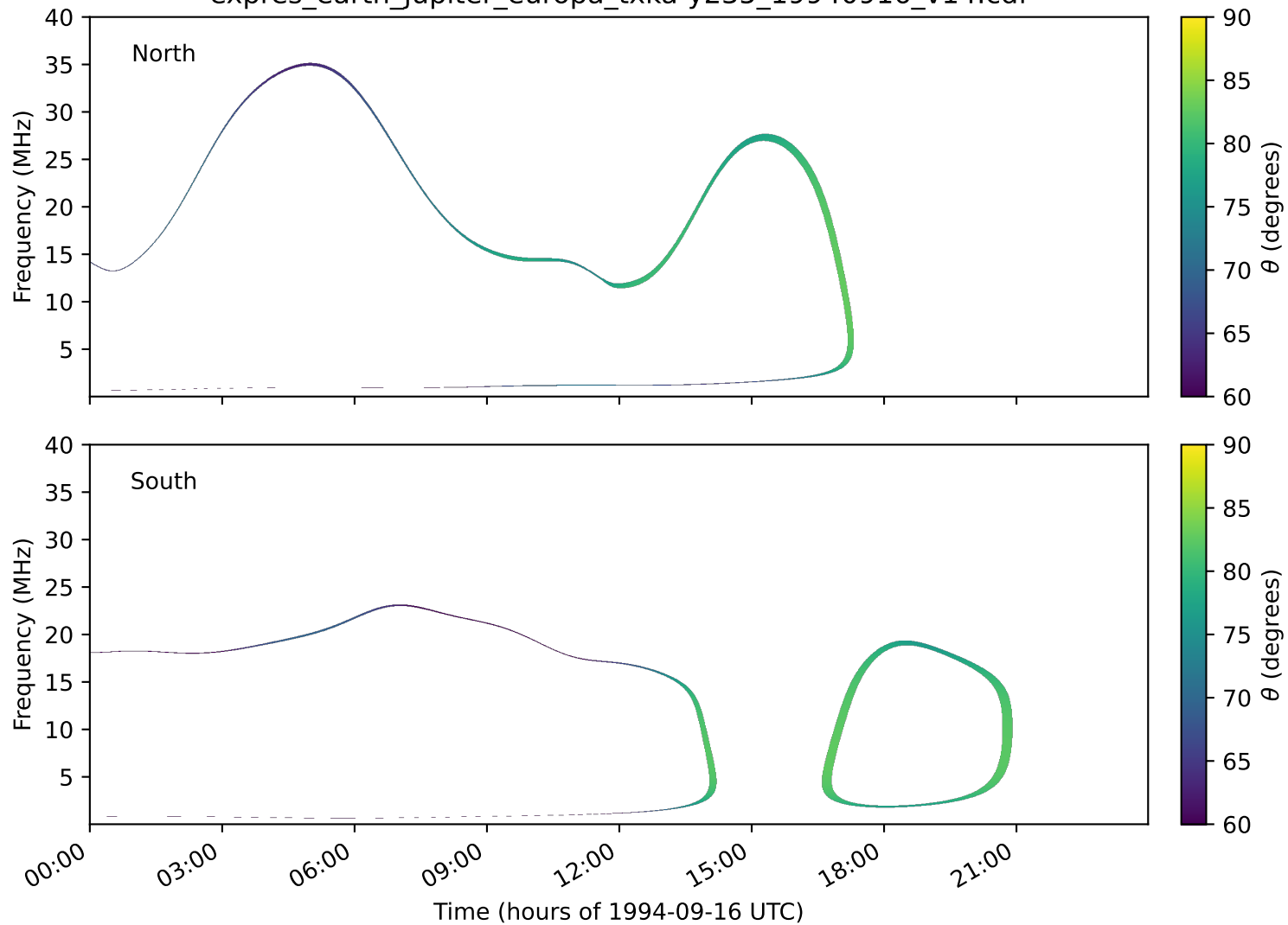
expres_earth_jupiter_europa_txka-y235_19940916_v14.cdf
