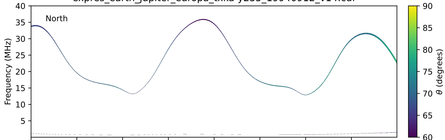
expres_earth_jupiter_europa_txka-y235_19940912_v14.cdf
