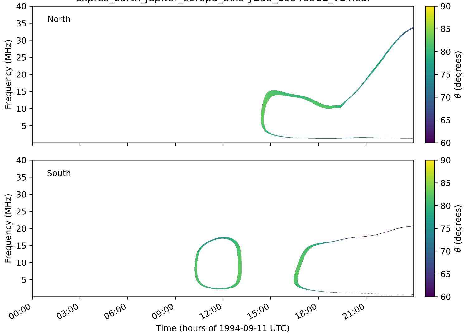
expres_earth_jupiter_europa_txka-y235_19940911_v14.cdf
