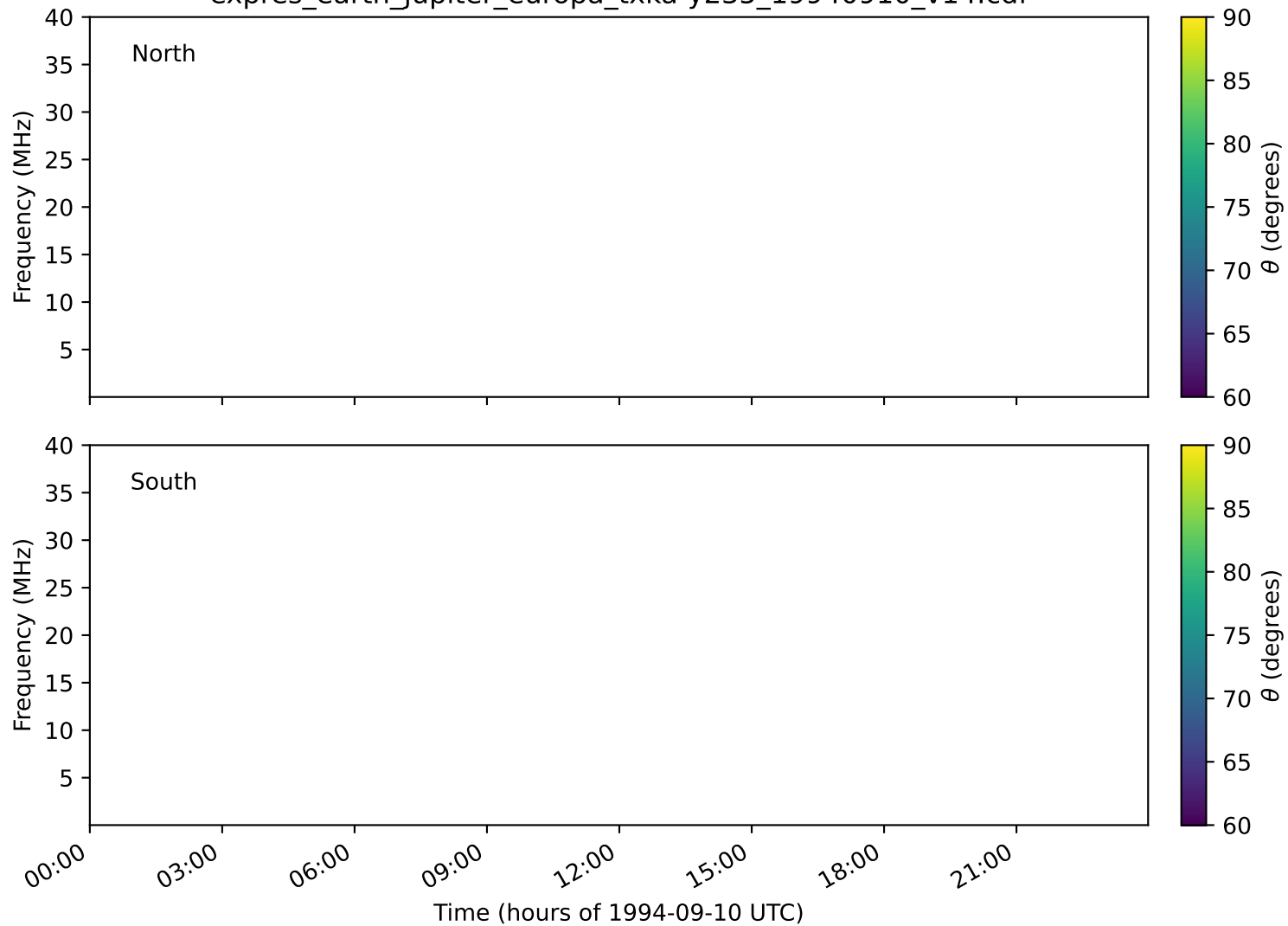
expres_earth_jupiter_europa_txka-y235_19940910_v14.cdf
