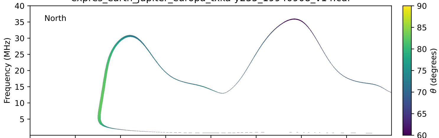
expres_earth_jupiter_europa_txka-y235_19940908_v14.cdf
