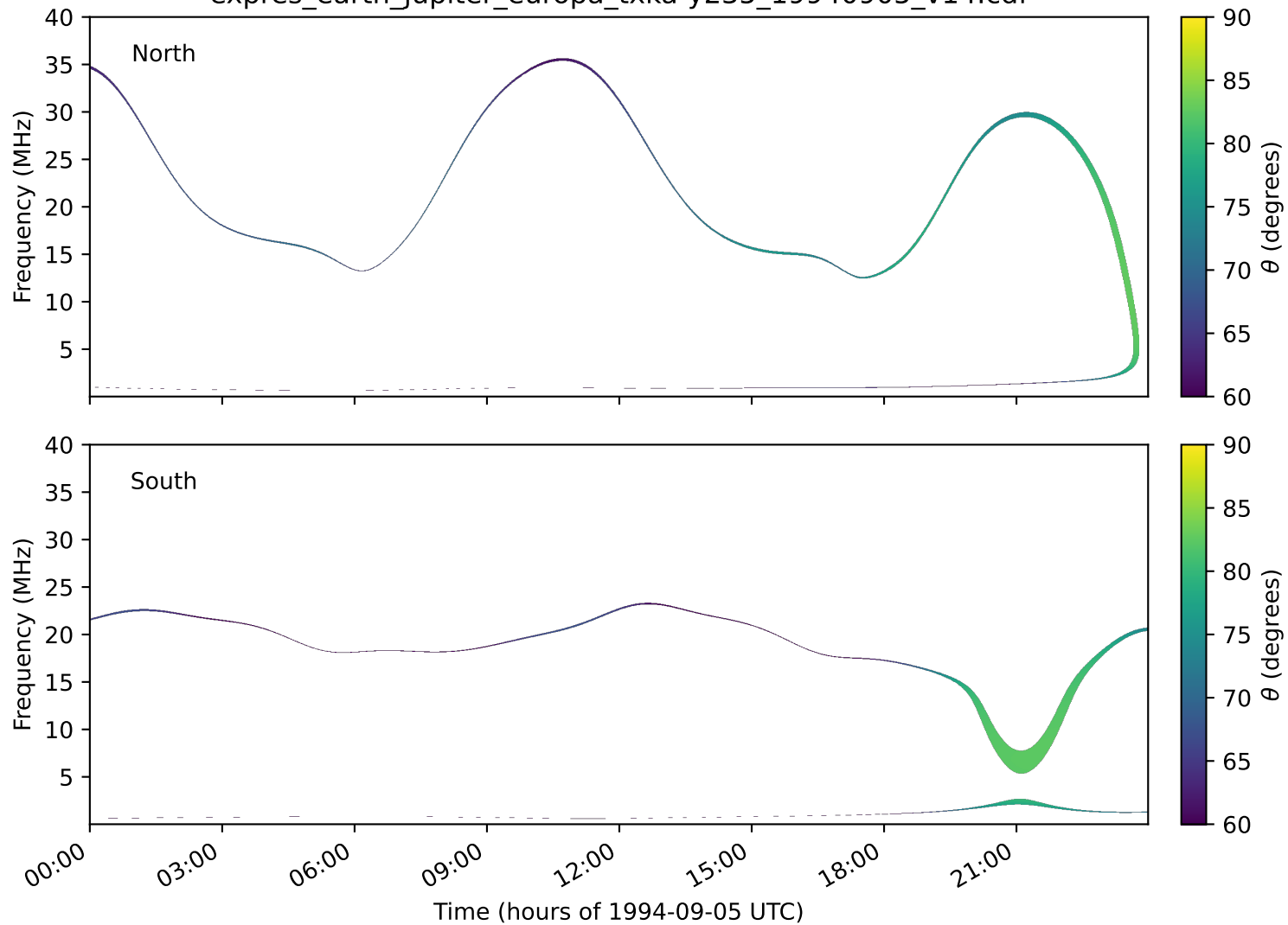
expres_earth_jupiter_europa_txka-y235_19940905_v14.cdf
