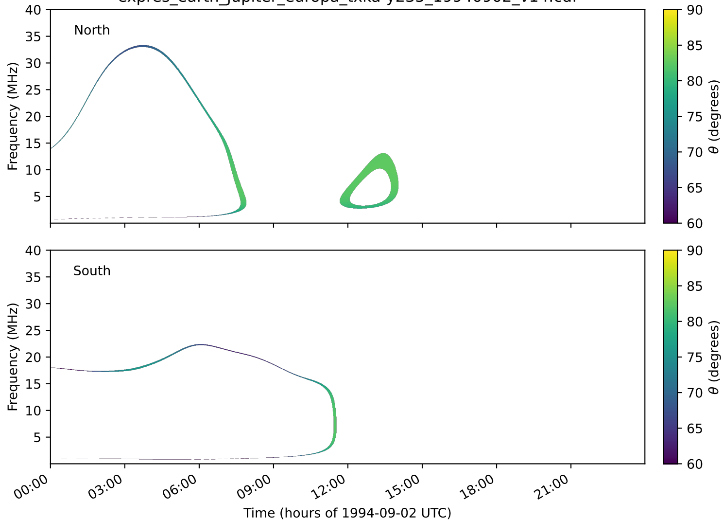
expres_earth_jupiter_europa_txka-y235_19940902_v14.cdf
