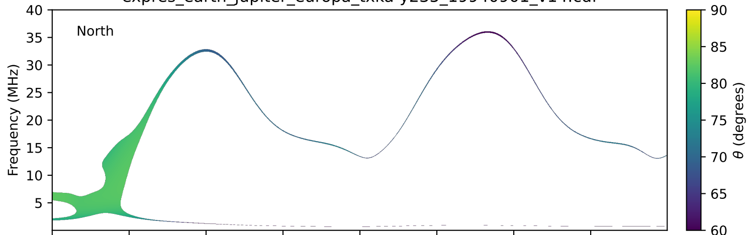
expres_earth_jupiter_europa_txka-y235_19940901_v14.cdf
