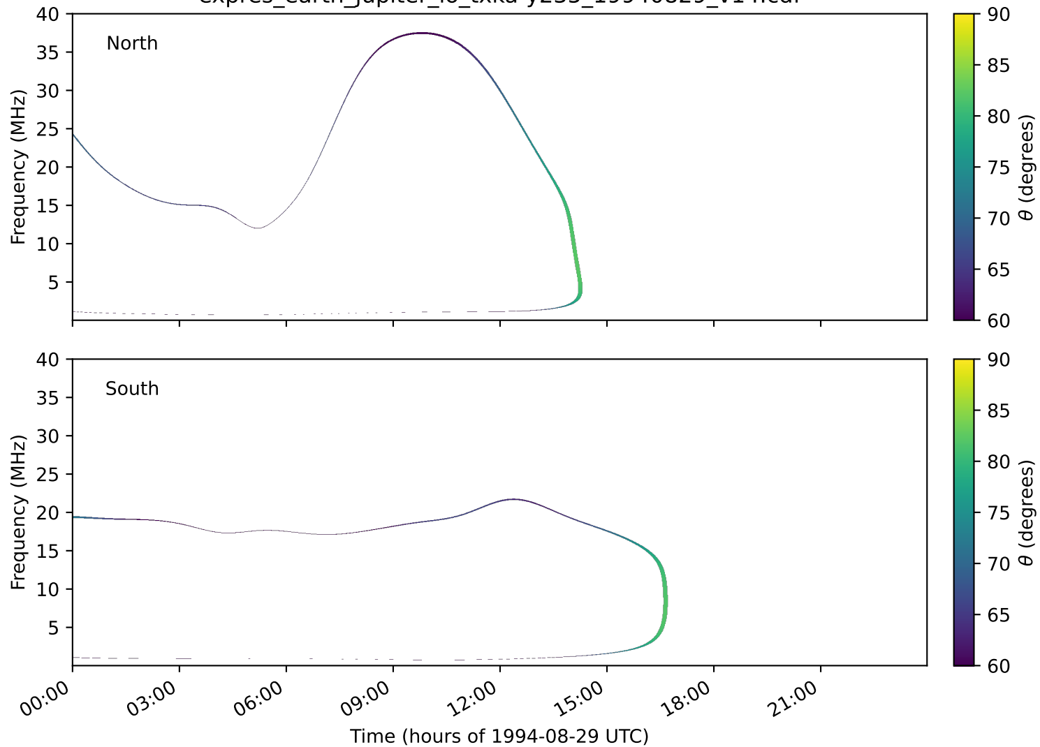
expres_earth_jupiter_io_txka-y235_19940829_v14.cdf
