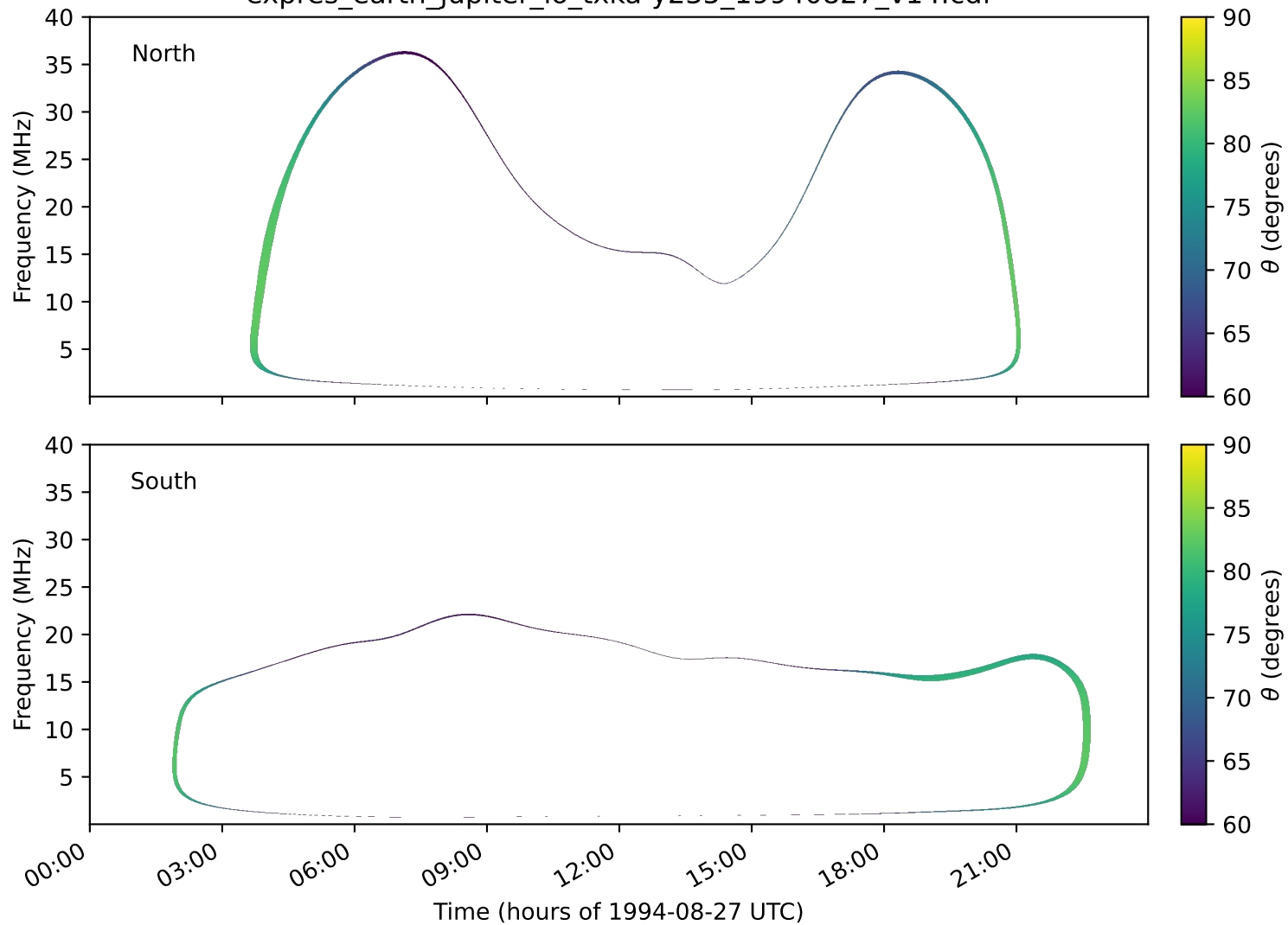
expres_earth_jupiter_io_txka-y235_19940827_v14.cdf
