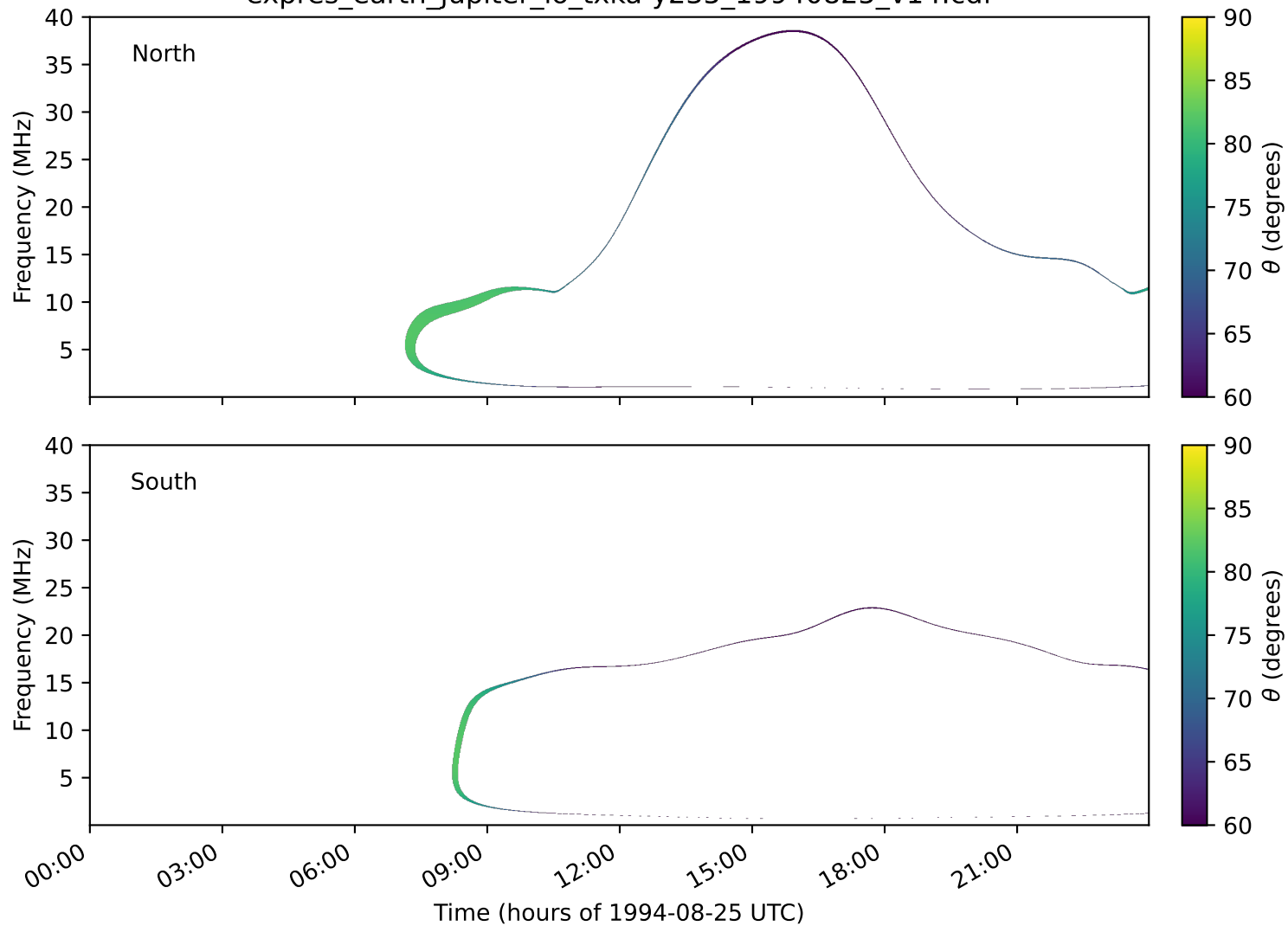
expres_earth_jupiter_io_txka-y235_19940825_v14.cdf
