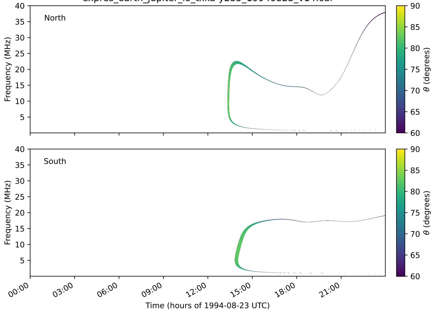
expres_earth_jupiter_io_txka-y235_19940823_v14.cdf
