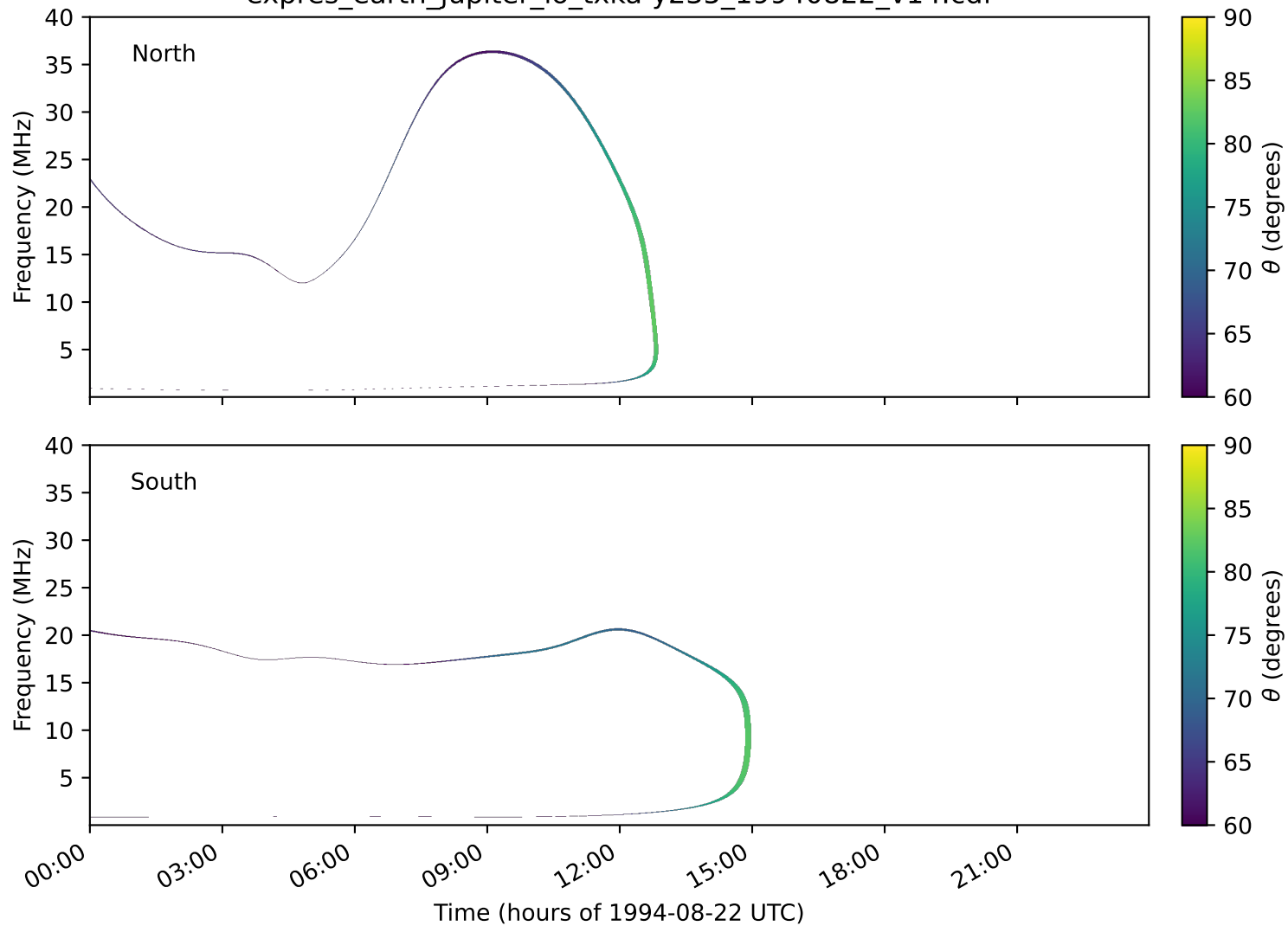
expres_earth_jupiter_io_txka-y235_19940822_v14.cdf
